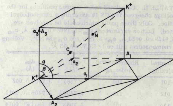
FIG. 4. Relation of the crystallographic unit cells for KCN III and KCN IV. \vec{a}_1 , \vec{a}_2 , \vec{a}_3 are the edges of the cubic cell for KCN III. \vec{A}_1 , \vec{A}_2 , and \vec{A}_3 are the edges of the C-centered monoclinic cell derived from the rhombohedral cell which results from the application of a small rhombohedral distortion to the cubic cell. The monoclinic cell for KCN IV may be pictured as the result of a rhombohedral distortion followed by a monoclinic distortion as described in the text. The C and N atoms, shown as lying along a [111] axis in the above figure, lie in ordered positions in the A_1A_3 plane in the monoclinic cell of KCN IV.
